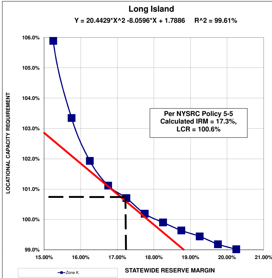
NYCA Locational ICAP Requirements vs. Statewide ICAP Requirements
