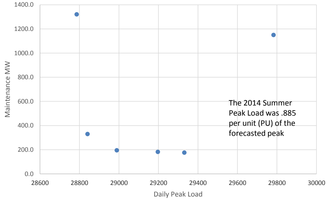
2014 Summer Maintenance VS Daily Peak Loads Loads > than .85 PU of Expected Summer Peak
