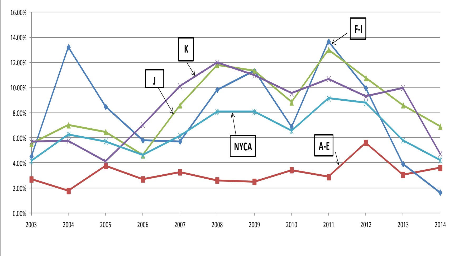
New York Annual Zonal EFORDs Weighted Values for Thermal and Large Hydro Units
