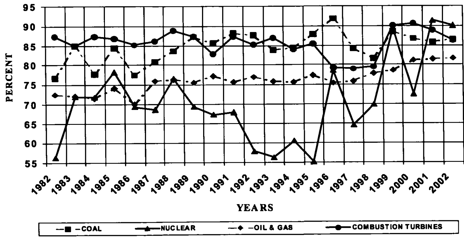
Figure A-6 NYCA EQUIVALENT AVAILABILITY BASED ON NERC-GADS DATA FROM 1982 - 2002 ANNUAL WEIGHTED AVERAGES FOR NUCLEAR, COAL, OIL & GAS, AND COMBUSTION TURBINES
