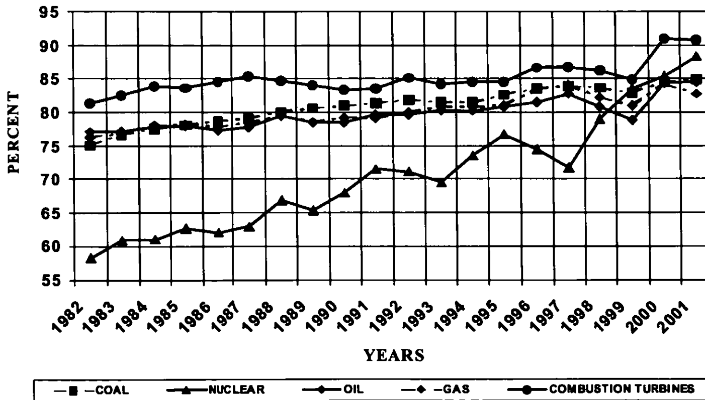
Figure A-7 NERC EQUIVALENT AVAILABILITY BASED ON NERC-GADS DATA FROM 1982 - 2001 ANNUAL WEIGHTED AVERAGES FOR NUCLEAR, COAL, OIL, GAS, AND COMBUSTION TURBINES
