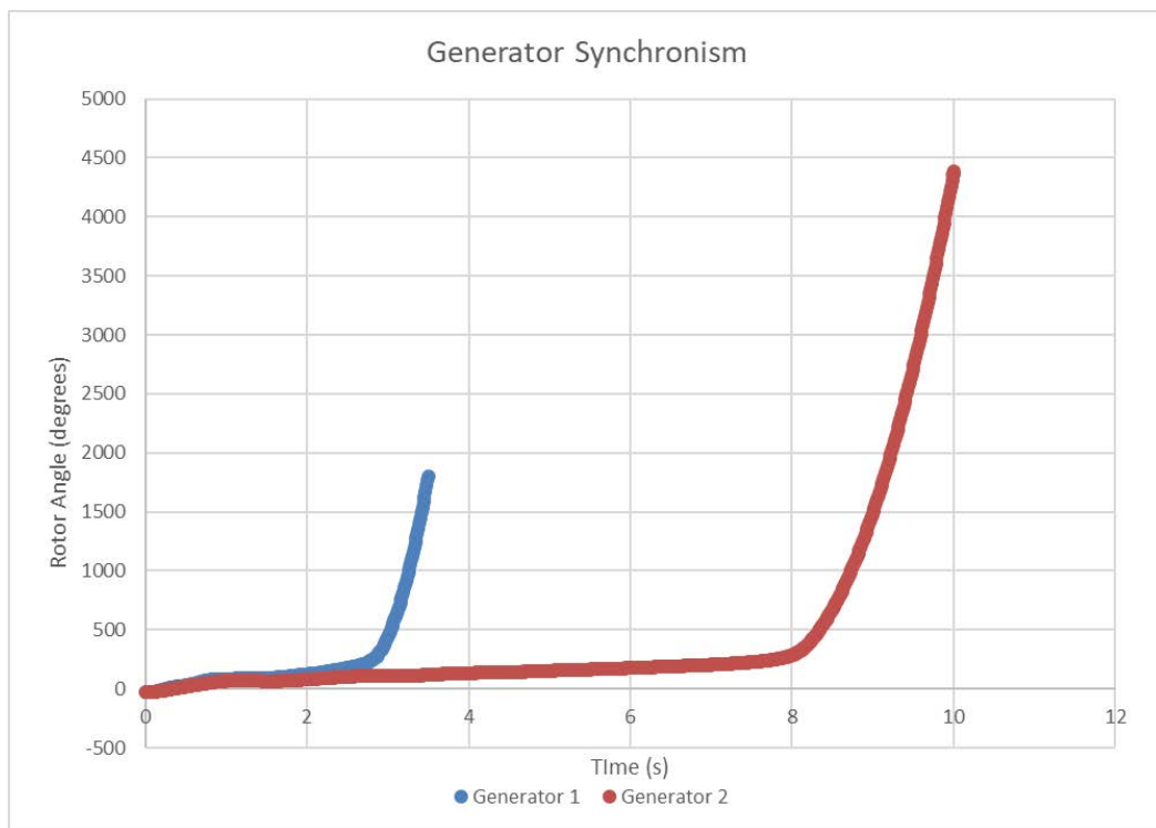
Figure 25: Generator Synchronism
