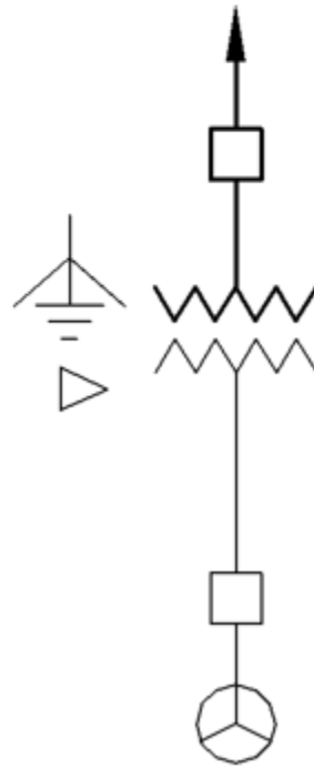
Delta-Wye Grounded Step-Up
