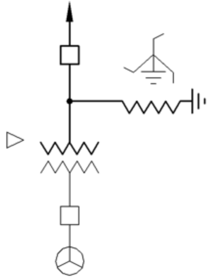
Zig-Zag Grounding Bank
