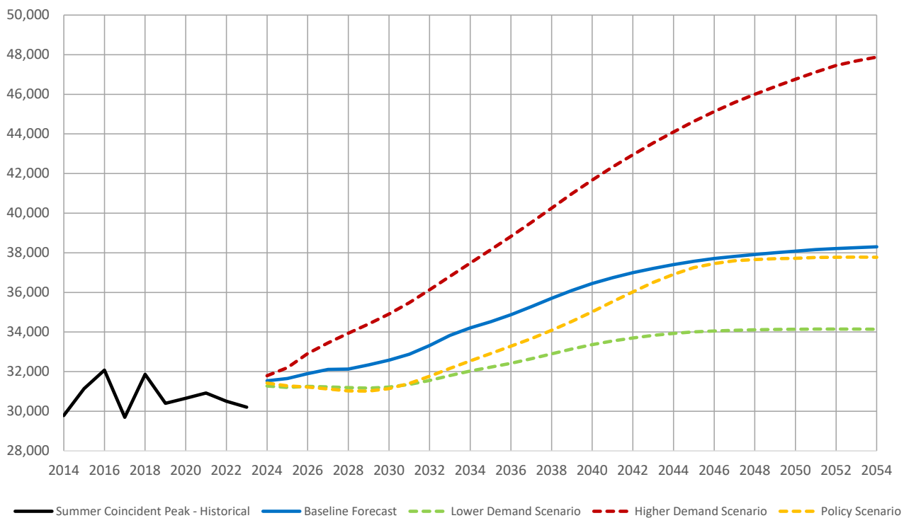
Figure I-2: NYCA Summer Peak Forecasts – Coincident Peak, MW
