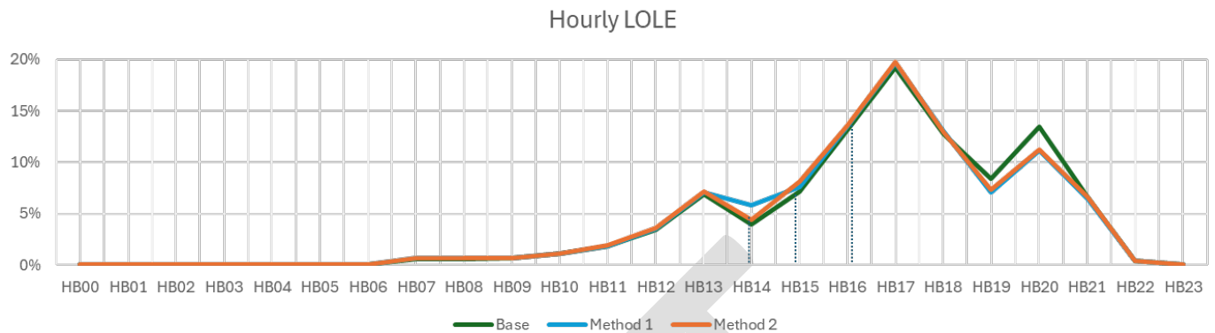
Figure 2: Hourly LOLE
