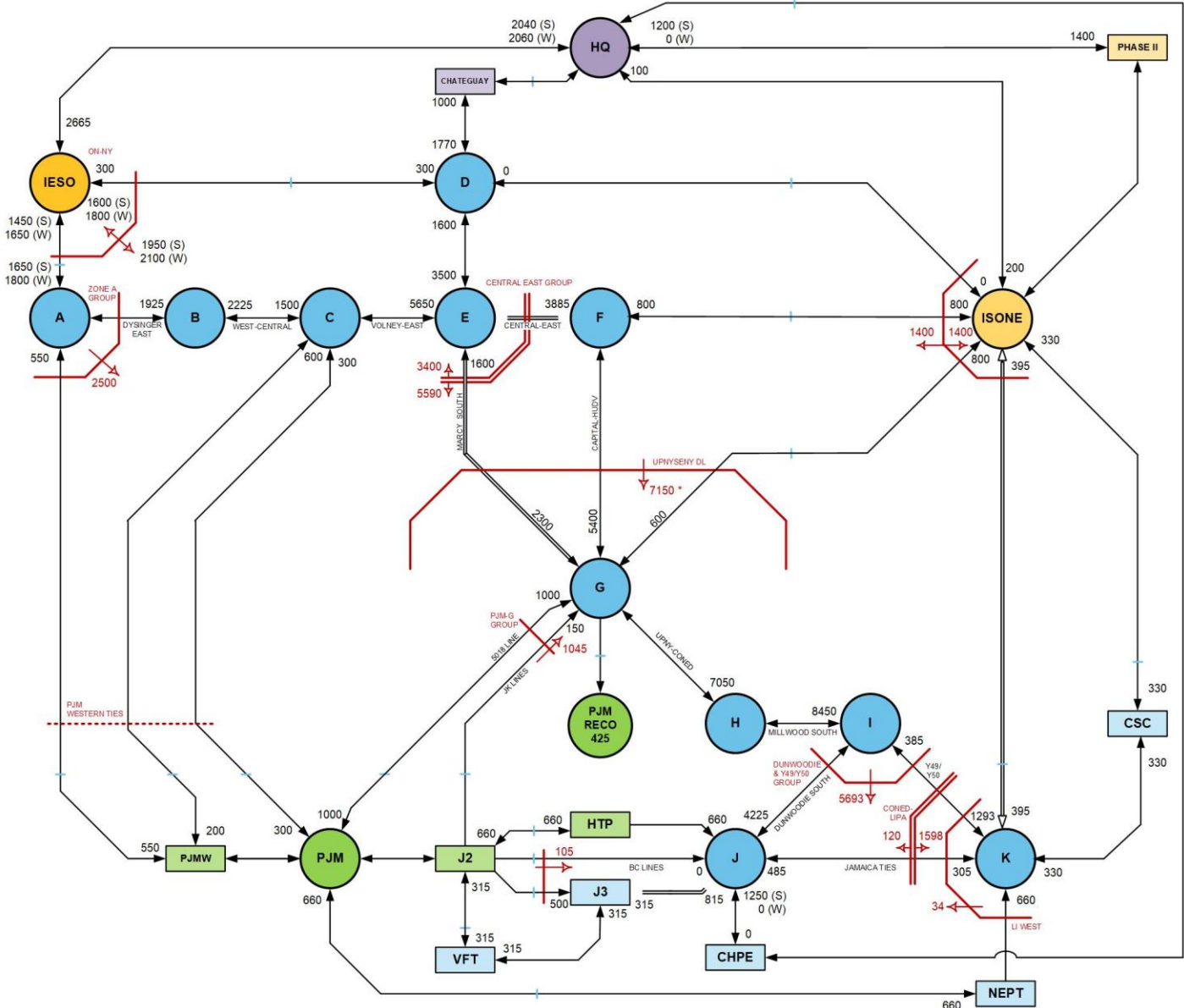
Figure A.10 2026-2027 IRM Topology
