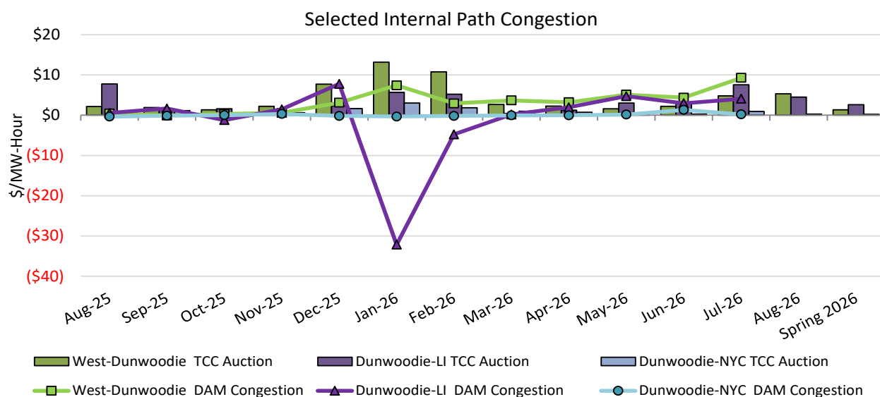
TCC Monthly Reconfiguration Auction vs. Monthly DAM Average with Spring 2026 Centralized TCC Auction Six-Month Average
