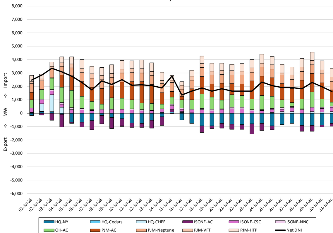
Daily Average Interchange by Proxy July 2026
